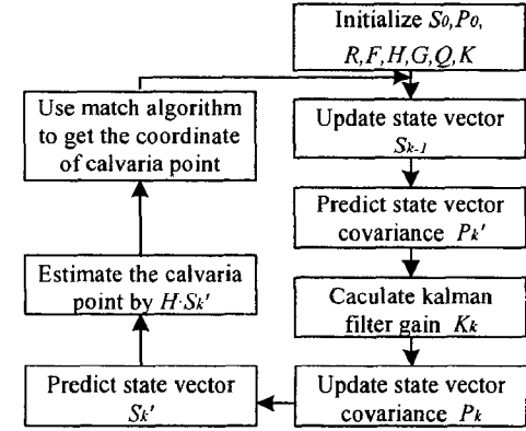
Figure 3. The flow chart of Kalman filter
