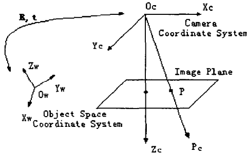
Figure 7. Projective transformation
