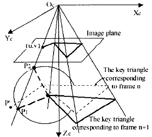
Figure 9. Ambiguity elimination in the subsequent frames
