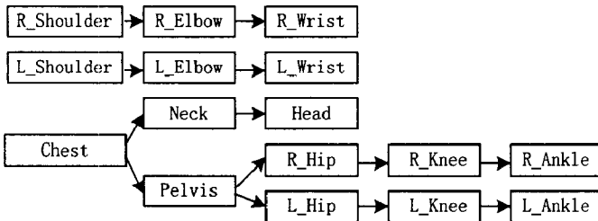
Figure 8. The solution order of 3D feature point
